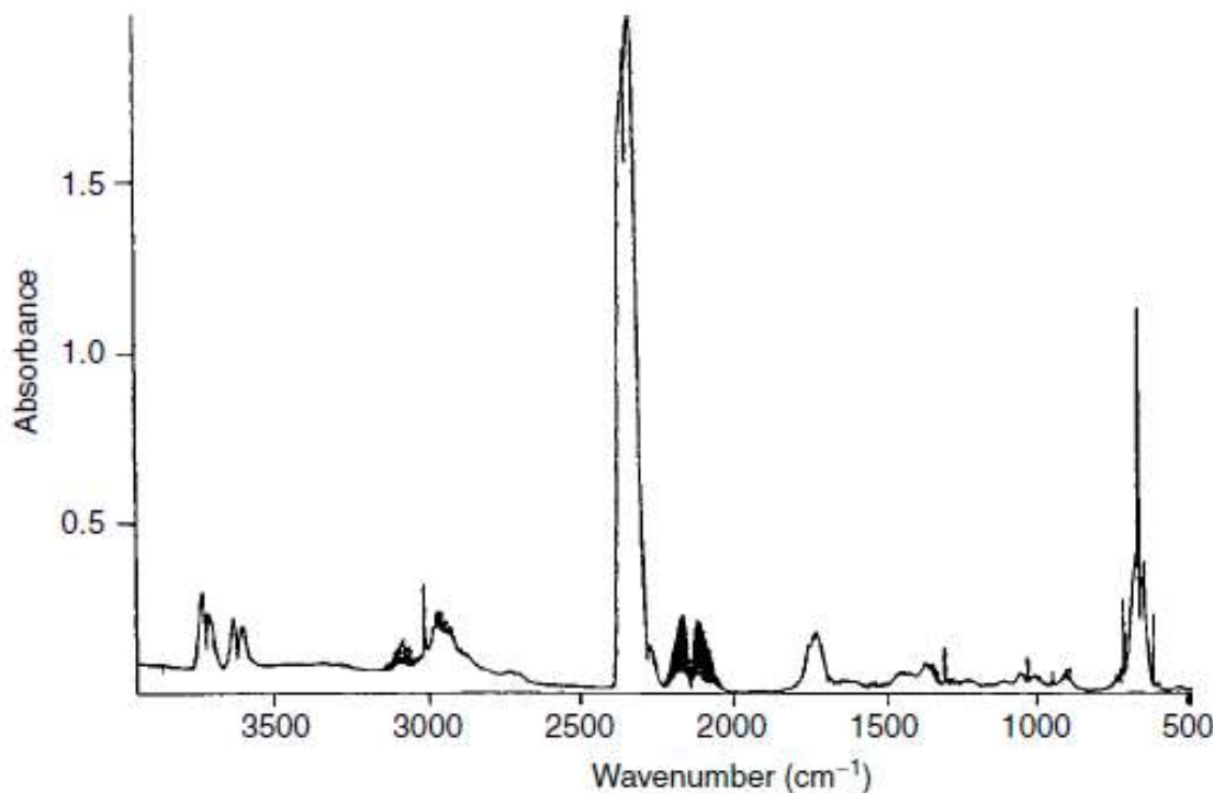
Figure 8.21 Infrared spectra of cigarette smoke (cf. SAQ 8.7) [35]. Used with permission from the Journal of Chemical Education , 78, No. 12, 2001, pp. 1665–1666; Copyright ©2001, Division of Chemical Education, Inc.
