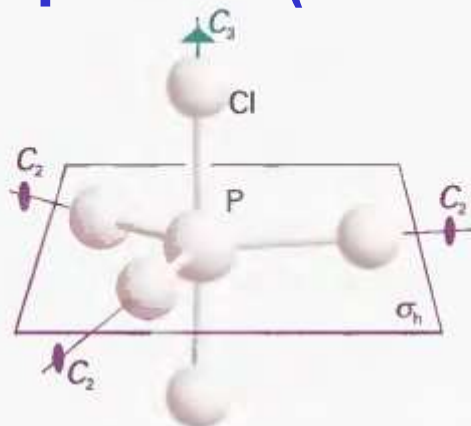
10 Phosphorus pentachloride, PCl 5 (D 3h )
