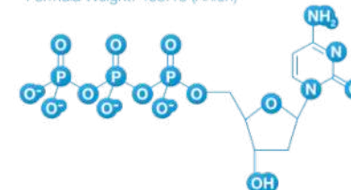
dCTP Formula: C_{10}H_{12}N_4O_{13}P_3 (Anion) Formula Weight: 463.15 (Anion)
