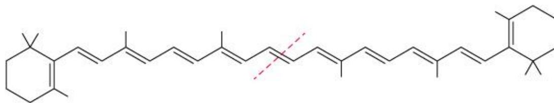
\beta -carotene
