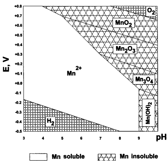
FIGURE 6.8. E – \text{pH} diagram for Mn.
