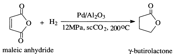
FIGURE 12.19. Hydrogenation using scCO 2 . (Source: Pillai and Sahle-Demessi, 2002).
