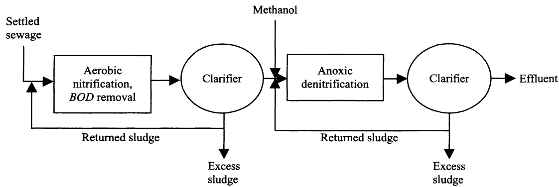
FIGURE 11.12. Double-sludge system for nitrogen removal.
